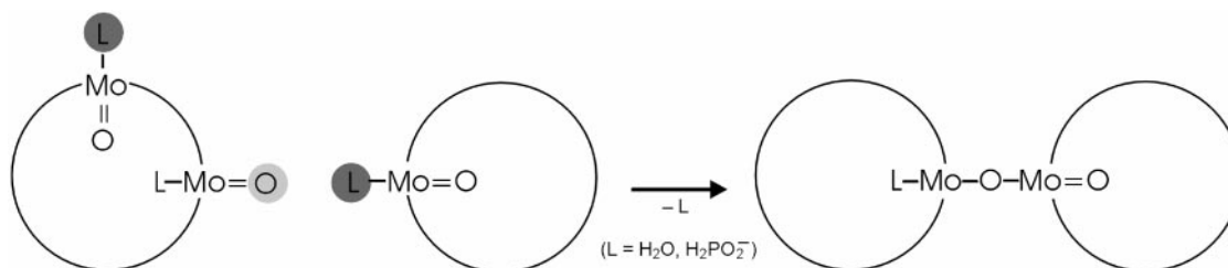
FIG. 7. Schematic representation of the basic assembly principle of the “giant-wheel”-shaped cluster units forming the networks and layers. The formation is based on the synergetically induced functional complementarity of the \{\text{Mo}_2\} units \text{O}=\text{Mo}(\text{L}) (e.g., \text{L} = \text{H}_2\text{O}, \text{H}_2\text{PO}_2^- ) on their surfaces.
